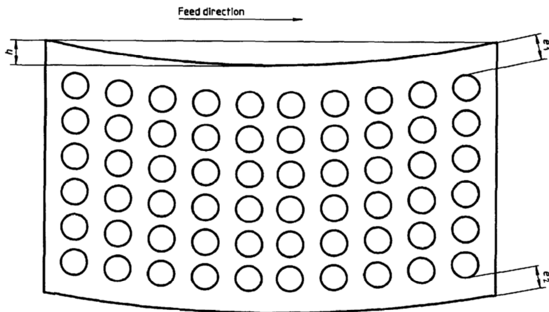
Figure 6 — Measurement of edge bow
