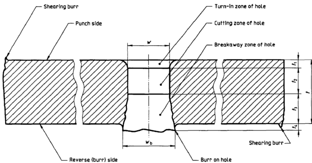
Figure 4 — Cross-section of perforated metal plate
