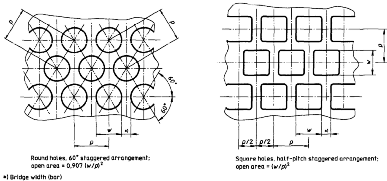
Figure 1 — Examples of hole arrangements
