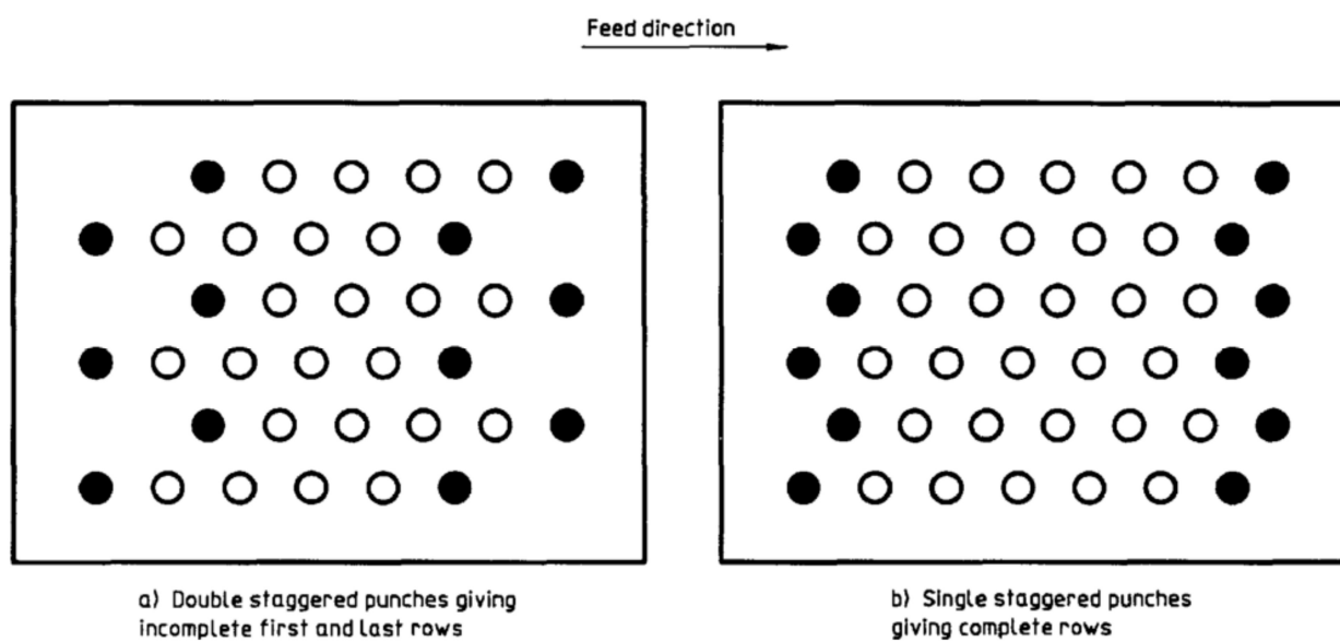
Figure 7 — Patterns of perforations caused by different tool arrangements (the positions of the punches in the tool are shown in black)
