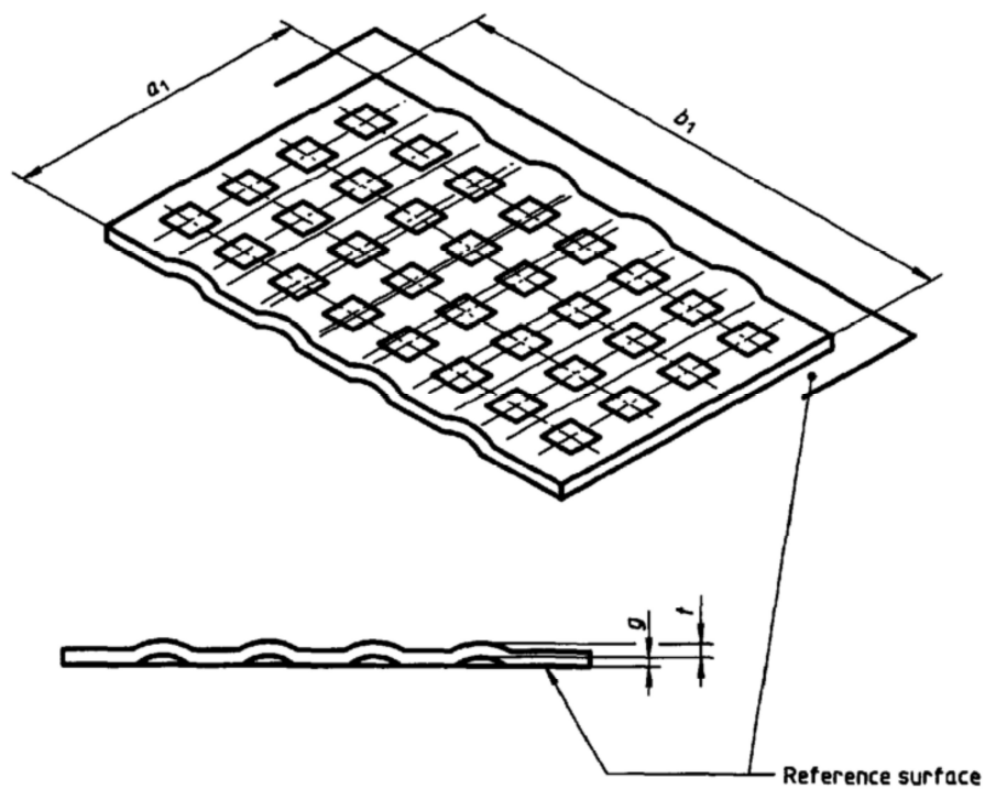
Figure 5 — Measurement of wavy edge
